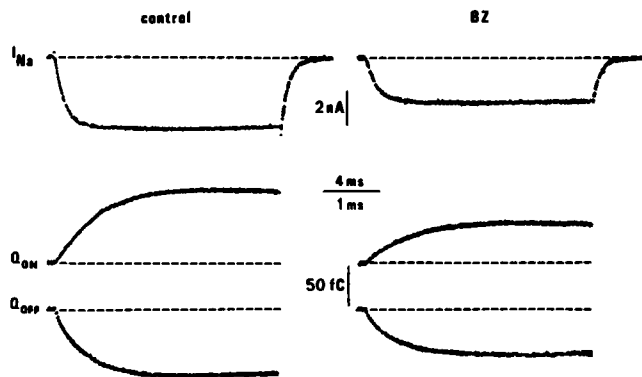
FIGURE 4 Na currents and ON and OFF charge movements recorded from a BTX-modified fiber during and after 16-ms pulses to -60 mV in control solutions (left) and in the presence of 1 mM benzocaine (right). Upper and lower horizontal scales correspond to I_{Na} and Q traces, respectively. Temperature: 13.5 – 14.5^\circ\text{C} . Fiber: 12–7–82.
